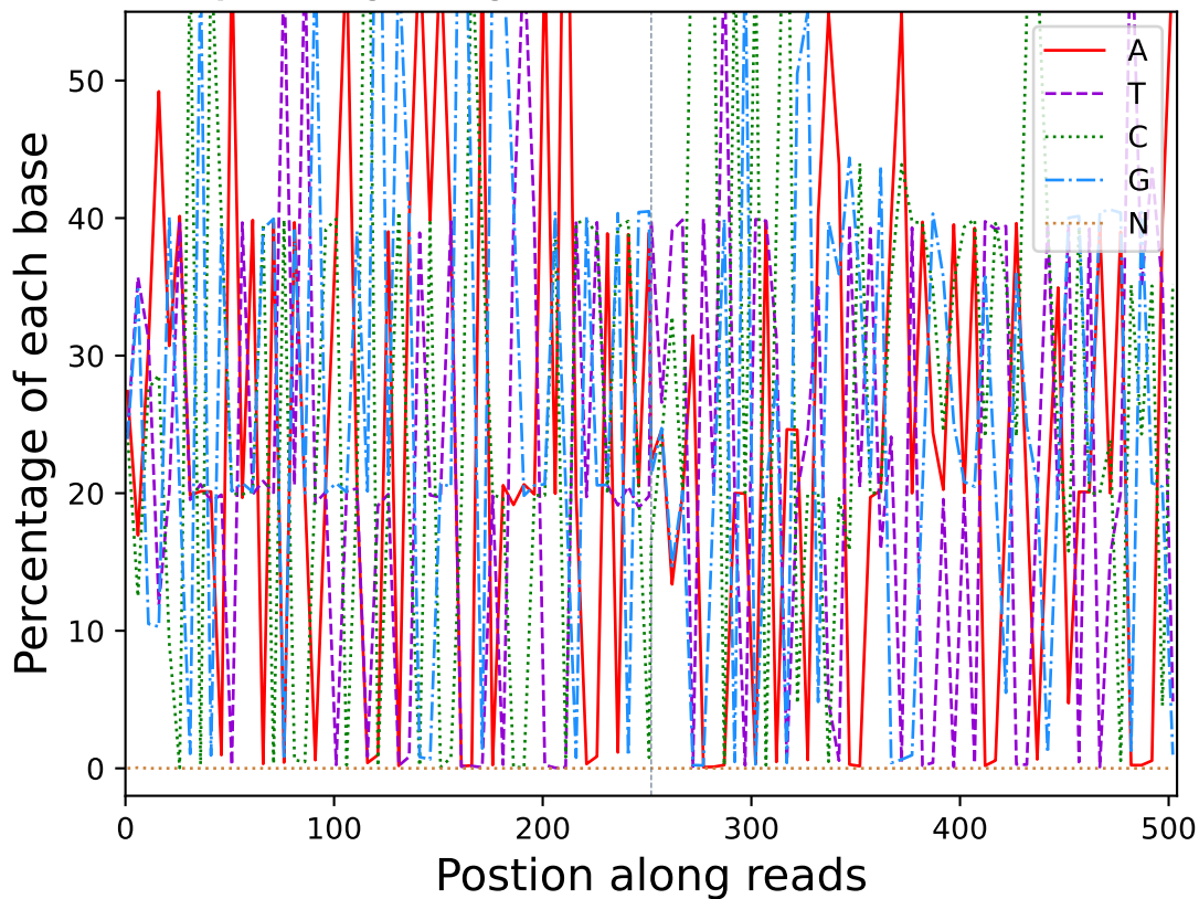
Base percentage along reads (R10112)
